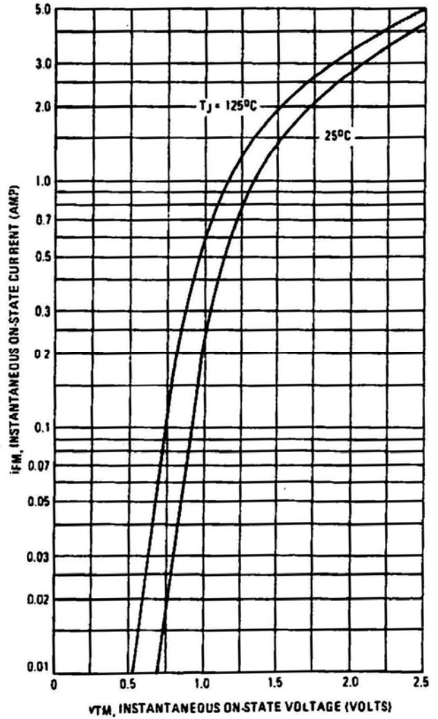
FIGURE 3 – FORWARD VOLTAGE
